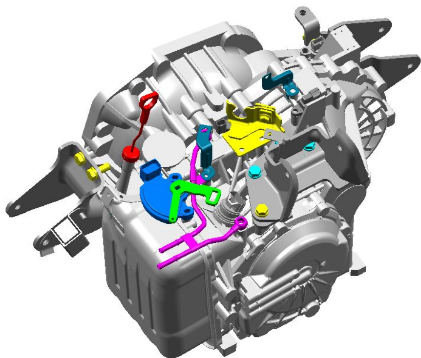
F4A42(θ-2.4L)
