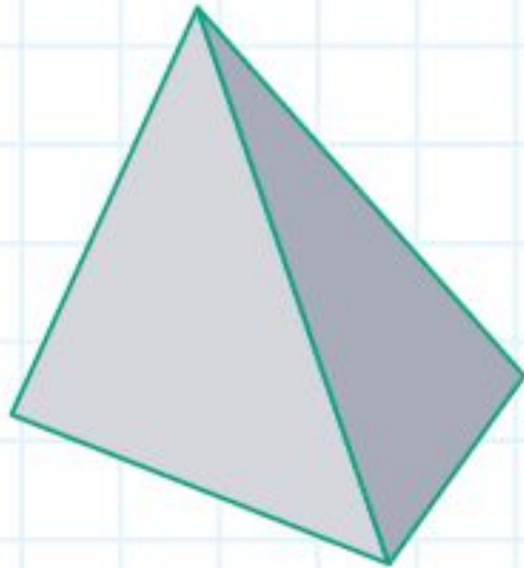
Regular Tetrahedron
