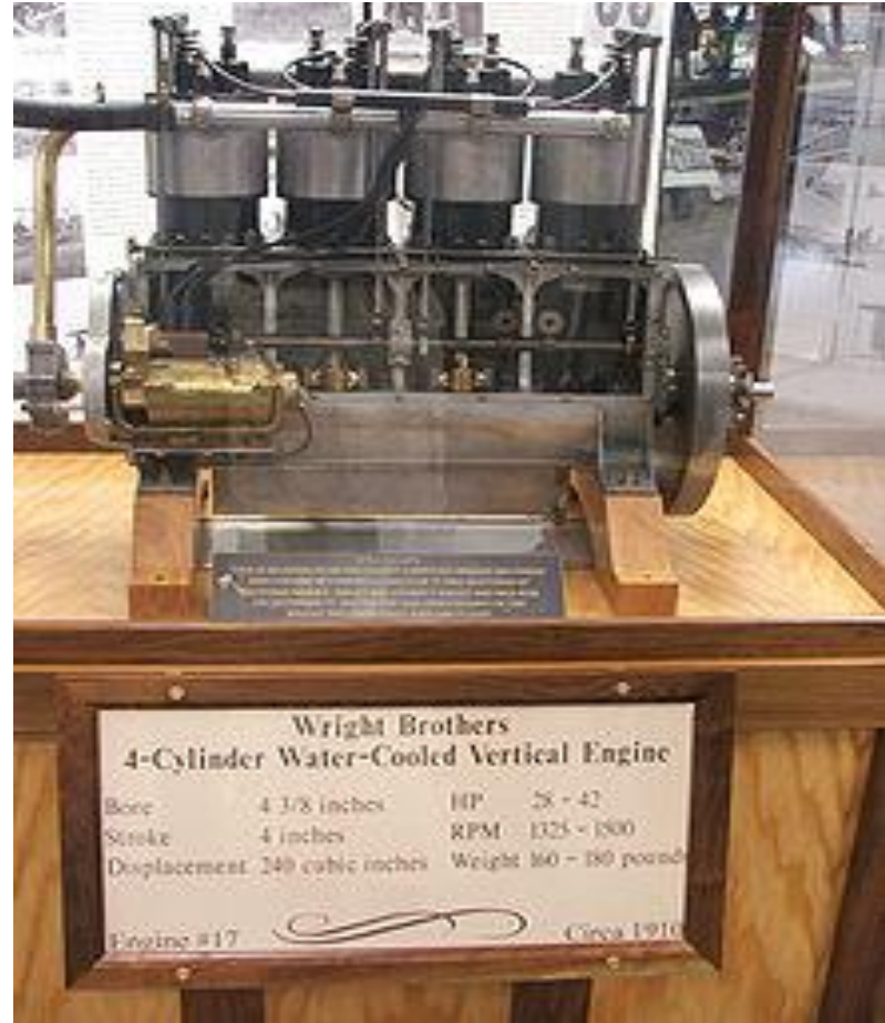
Wright Brothers 4-Cylinder Water-Cooled Vertical Engine
