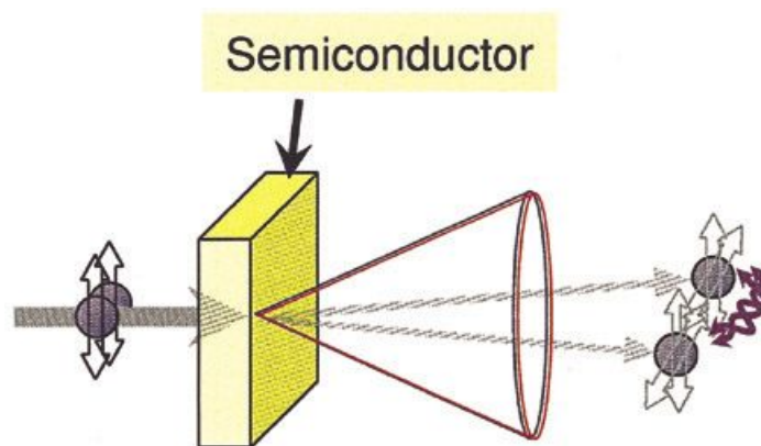
Entangled photon pair
