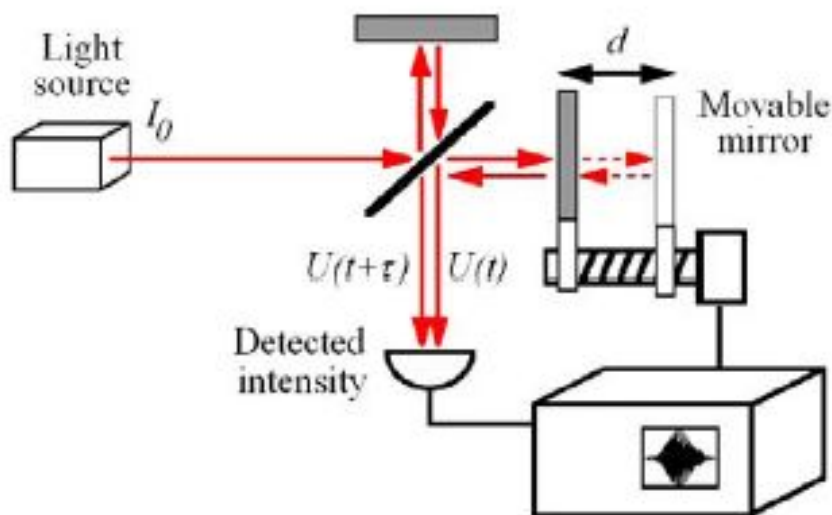
Michelson interferometer
