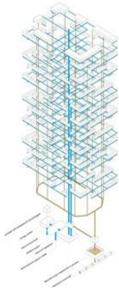
WATER SUPPLY SYSTEM
