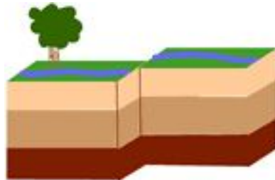
Strike-slip
