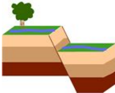
Normal
