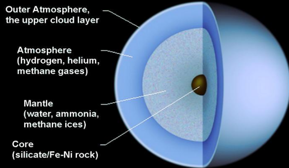
Internal Structure of Uranus
