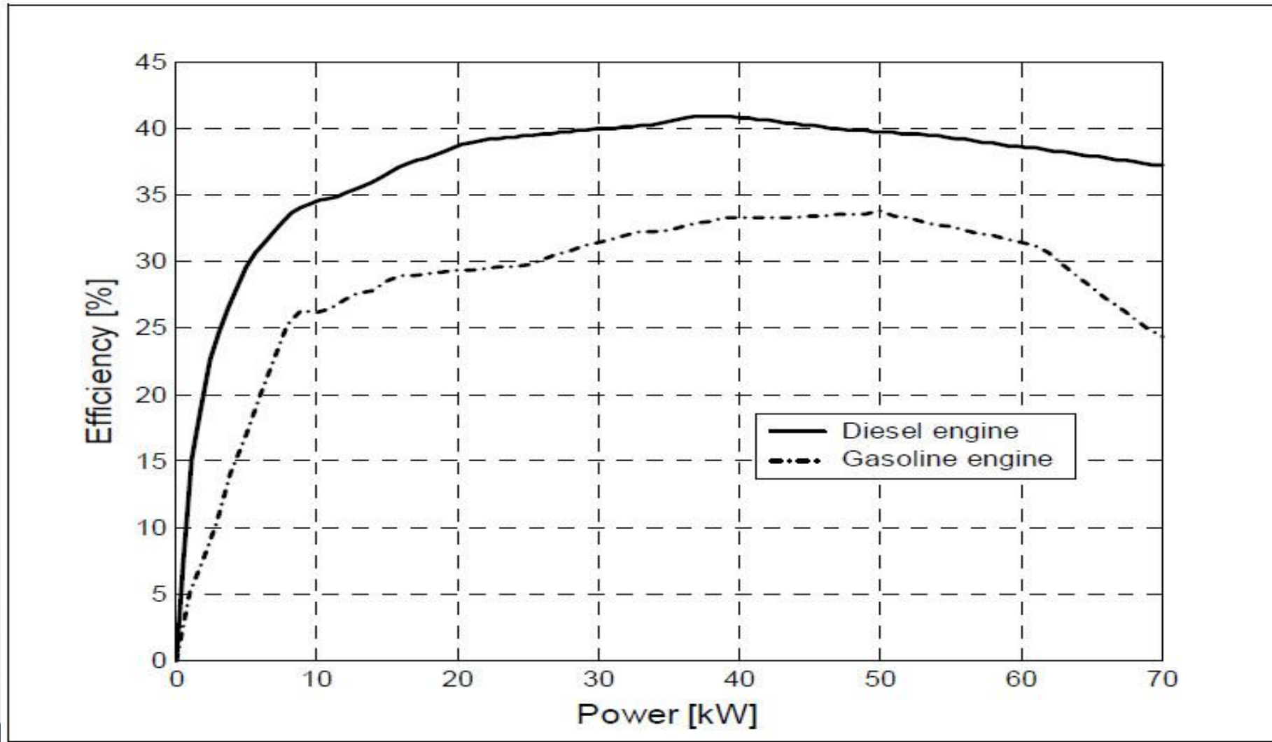
Graph power diesel and petrol engines
