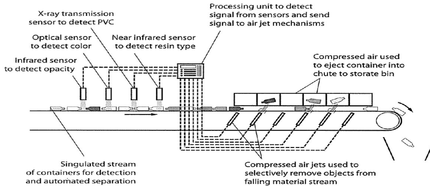
FIGURE 8.34 Systems for automated separation of solid waste components: (a) binary sorting device, and (b) an array of sensors for material identification.
