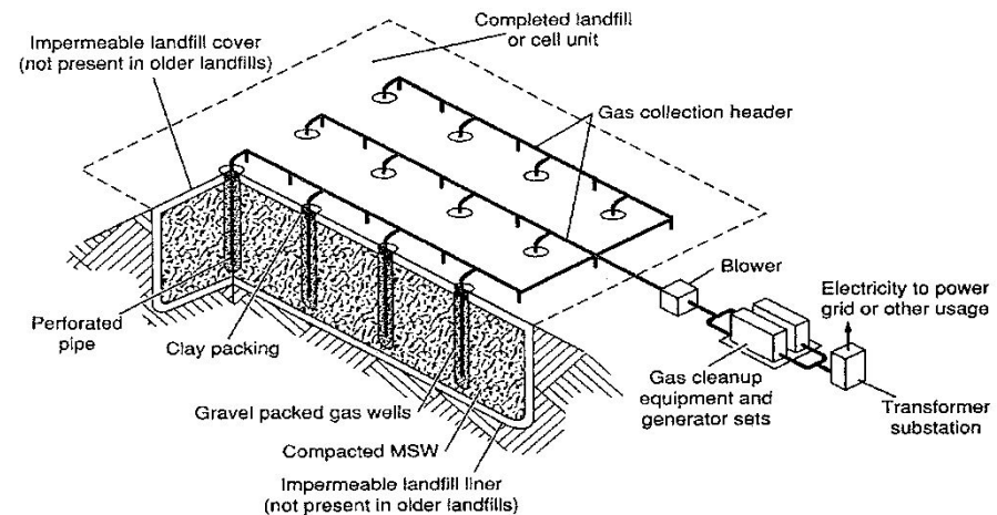
FIGURE 14.9 Landfill gas recovery system using vertical wells.
