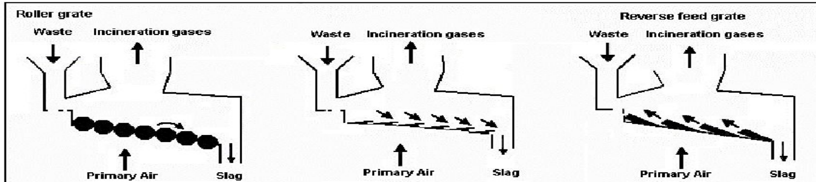
Figure 4.3: Different Grate Types Source [1, UBA, 2001]
