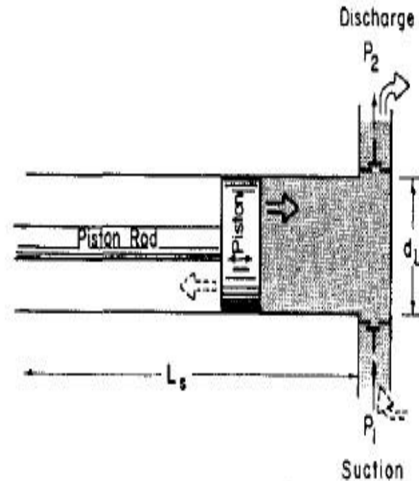
(b) Single-acting (triplex) design.
